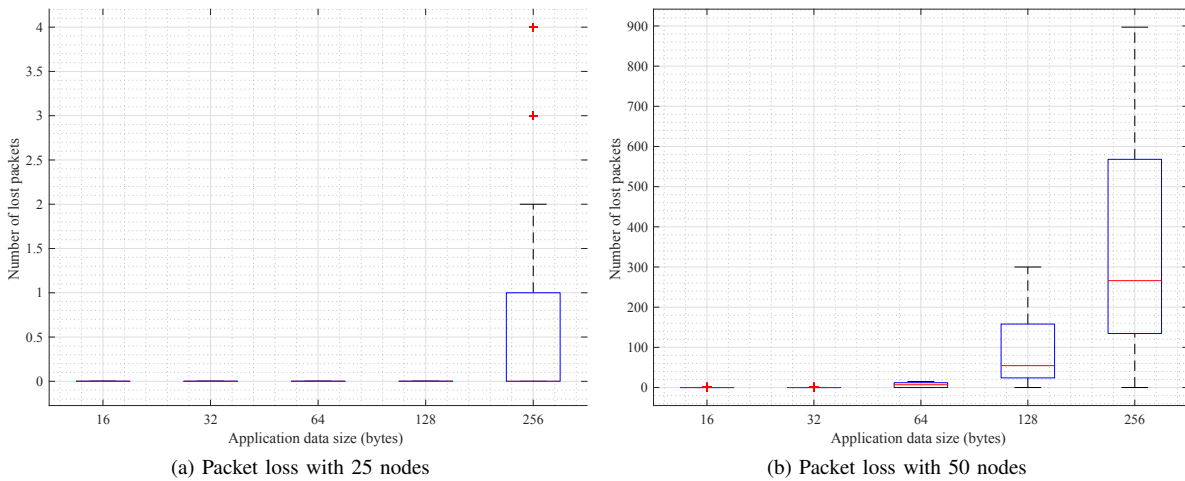
Figure 5: Packet loss vs data size over 6LoPLC network in buildings with 25 and 50 nodes
