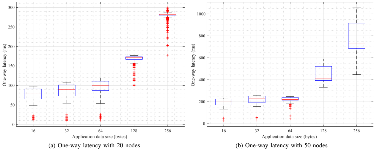
Figure 4: Latency vs number of payload size for various number of nodes
