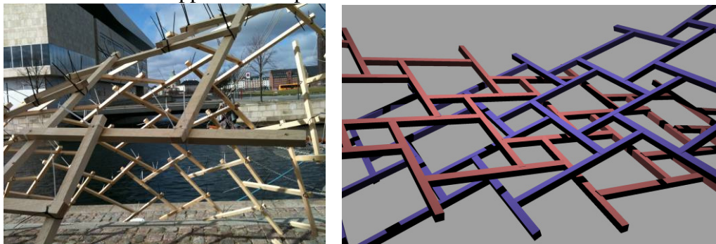
Figure 10 and b: The RF shell – detail of Physical and, CAD model
