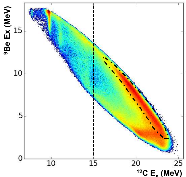
FIG. 3. (color online) Dalitz plot for the 26 MeV beam data. Natural parity states associated with {}^{12}\text{C} breakup appear as vertical bands and {}^9\text{Be} states form broad, horizontal bands. Neutron transfer events and subsequent breakups of the {}^5\text{He}_{\text{g.s.}} form the diagonal locus which is surrounded by the dot-dashed line. Only data to the right of the vertical dashed line were considered for further analysis in order to minimise contributions from {}^{12}\text{C} breakups.
