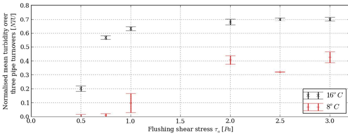
Figure 2: Results of laboratory studies into discolouration material regeneration (previously unpublished). Material layers were developed over 28 days under a steady boundary shear stress of 0.1\text{ Pa} ( 0.2\text{ L} \cdot \text{s}^{-1} ) at 8^\circ\text{C} and 16^\circ\text{C} . These layers were then eroded through imposing a series of discrete increases in shear stress.
