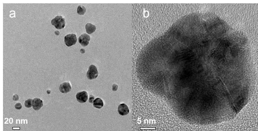
Figure 12. (a) TEM and (b) HRTEM image for Ag-Pd alloy NPs synthesized by simultaneous reduction of \text{Ag}(\text{NO}_3) and \text{Pd}(\text{NO}_3)_2 with HQ.
