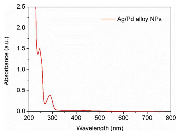
Figure 11. UV-vis spectrum of Ag-Pd alloy NPs synthesized by simultaneous reduction of \text{Ag}(\text{NO}_3) and \text{Pd}(\text{NO}_3)_2 with HQ. The solution was diluted for 10 times prior characterisation.
