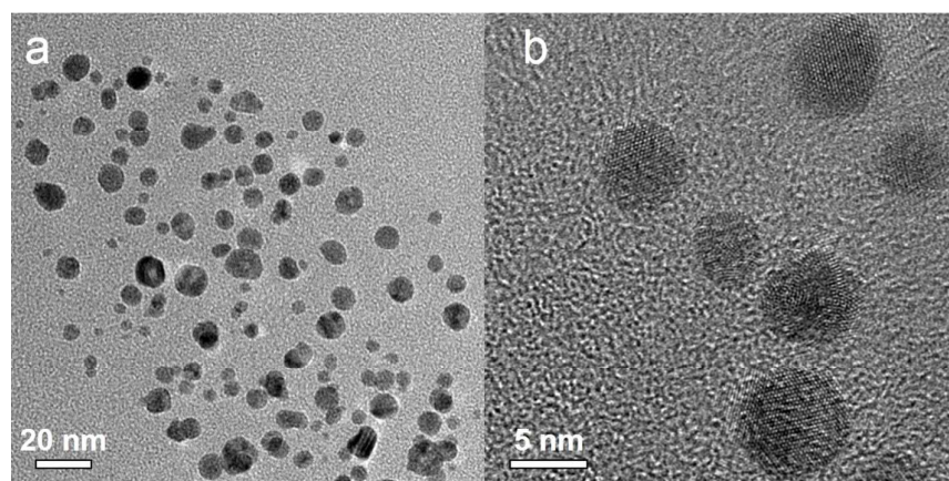
Figure 9. (a) TEM and (b) HRTEM images of nanoparticles synthesised using only \text{Pd}(\text{NO}_3)_2 in Reactor 3 and HQ in Reactor 4.
