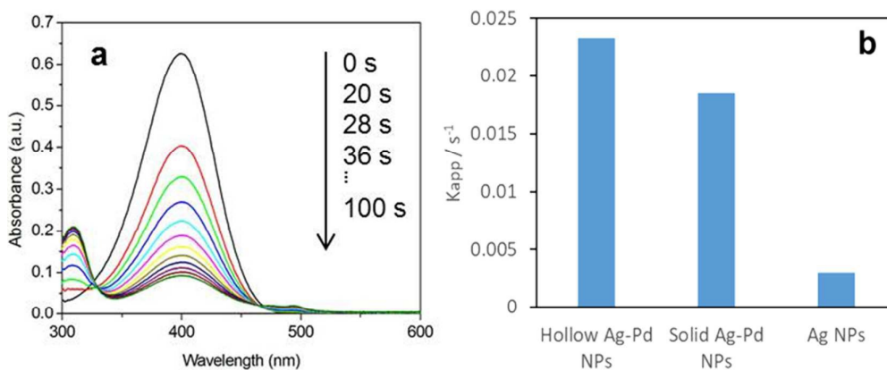
Figure 15. (a) Time-dependent UV-vis absorption spectra of the catalytic reduction of 4-nitrophenol to 4-aminophenol by an excess amount of \text{NaBH}_4 by hollow Ag-Pd NPs synthesised in 3 CFI reactors connected in series, using \text{Pd}(\text{NO}_3)_2 as precursor. (b) Average kinetic constant ( K_{\text{app}} ) value of hollow alloy Ag-Pd, solid alloy Ag-Pd (synthesised by simultaneous reduction with HQ) and Ag NPs (seeds).
