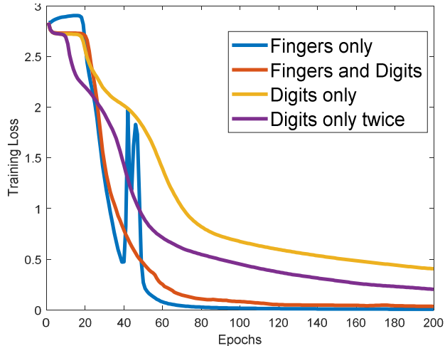
Figure 6. Training Loss for each epoch.
