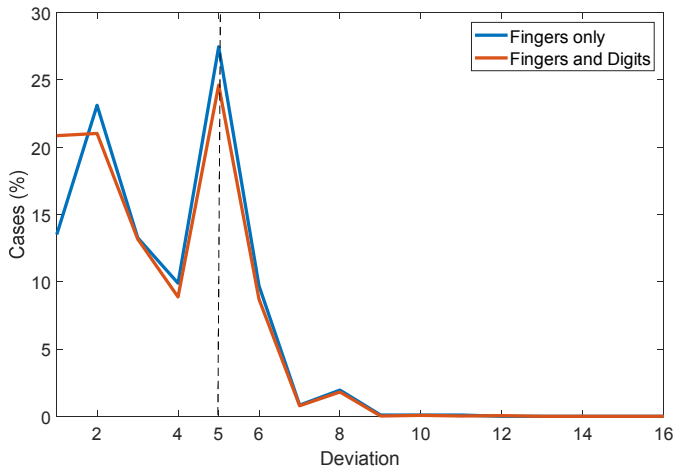
Figure 7. Absolute deviation from the correct addition. Cases are in percentage of the total number of errors. A larger number of split-five errors is evident as also observed in studies with human beings [5]–[7].
