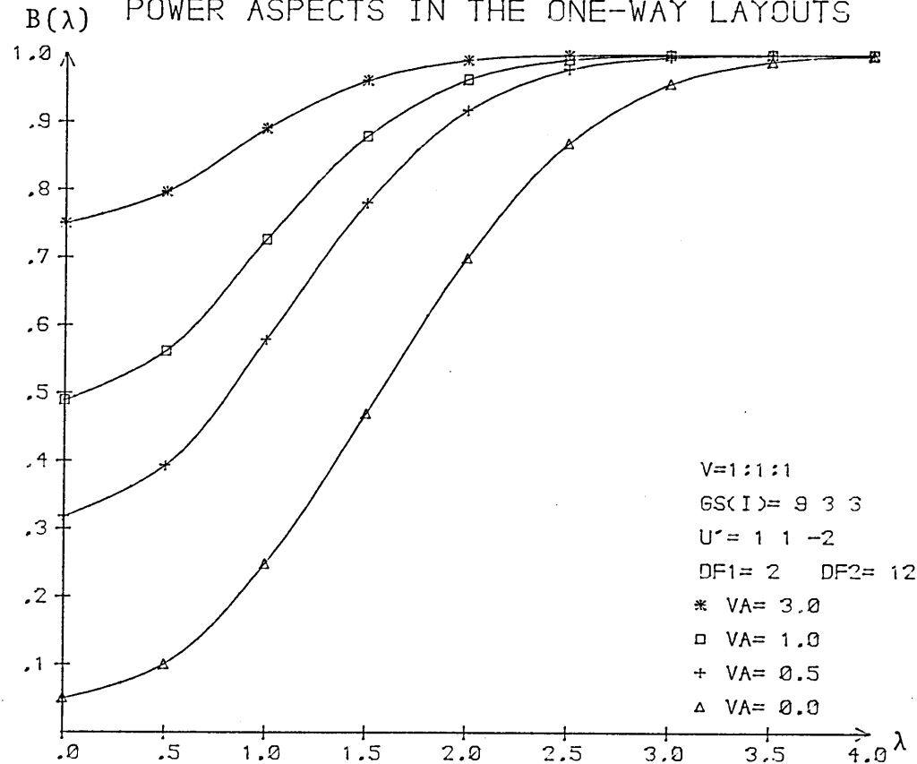
FIG. 2.2.7 EFFECTS OF VARIABILITIES OF TREATMENT MEANS ABOUT THEIR TRUE MEANS ON POWER.
