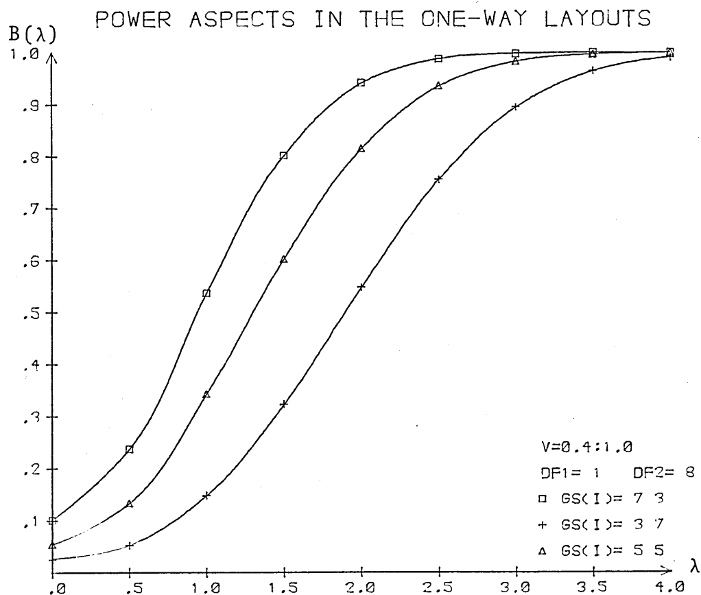
FIG. 2.1.7 EFFECTS OF GROUP SIZES ON POWER.
