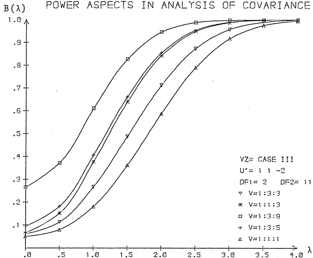
FIG. 4.3 EFFECTS OF UNEQUAL ERROR VARIANCES ON POWER.
