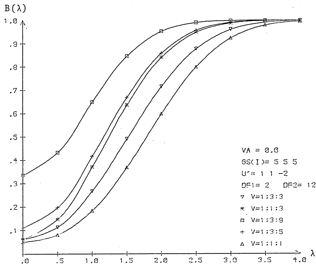
FIG. 2.1.4 EFFECTS OF UNEQUAL GROUP ERROR VARIANCES ON POWER.
