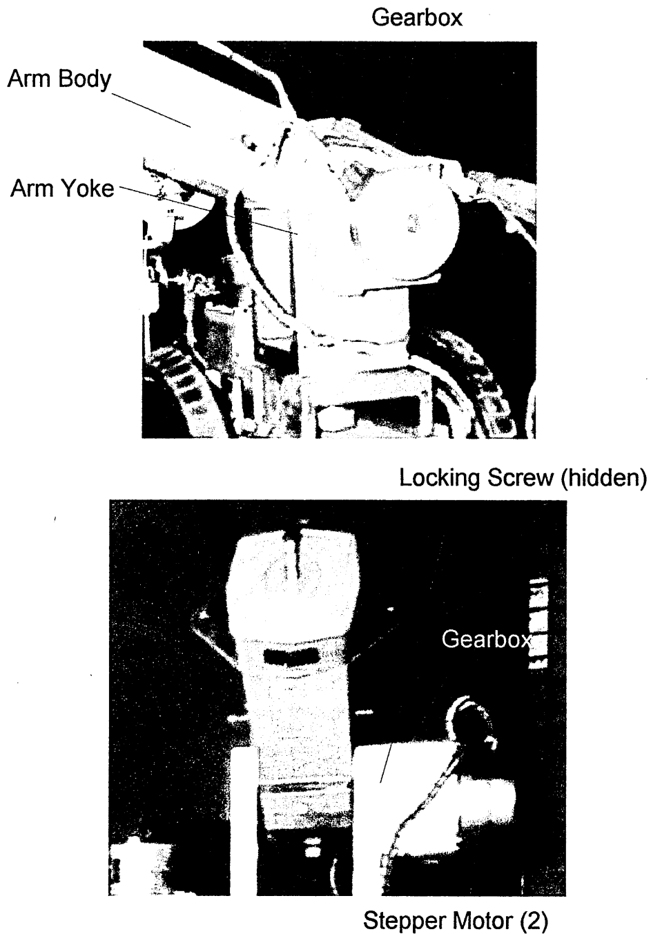
Figure 4.15: Joint 2 Motor Configuration
