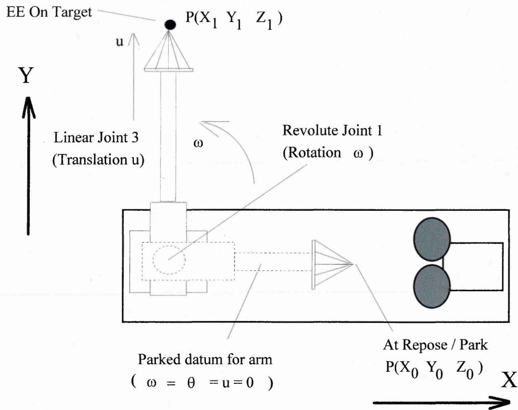
Figure 3.5a: Proposed Arm Configuration - Plan
