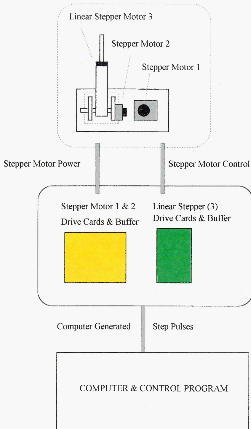
Figure 4.20: Arm Control Modules & Overview
