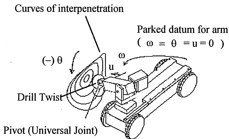
Figure 3.8: GRASP Generated Tractor/Arm Model and Target
