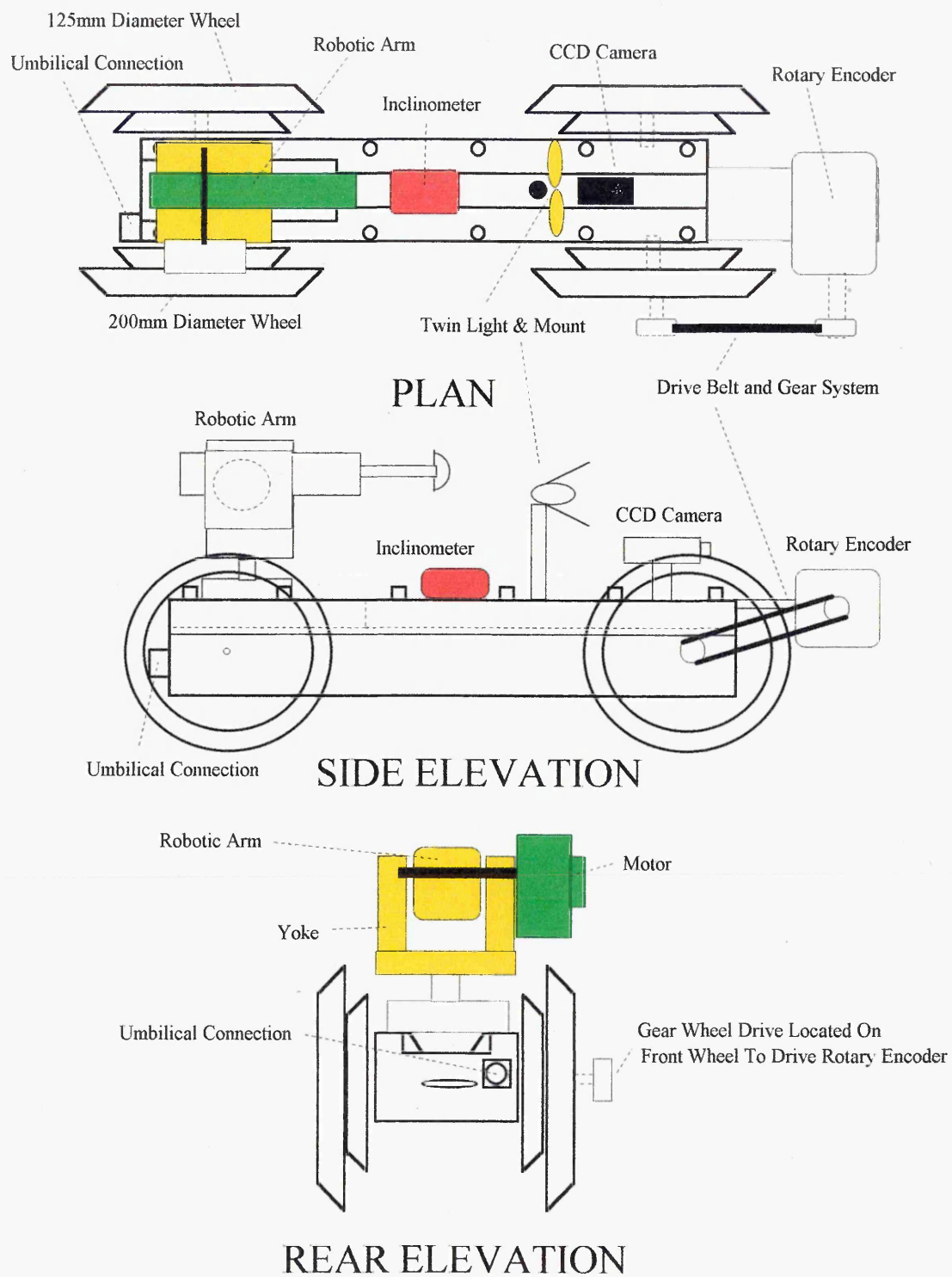
Figure 1.9: Diagrammatic Sketch Of Proposed Retro Fit Sewer Robot
