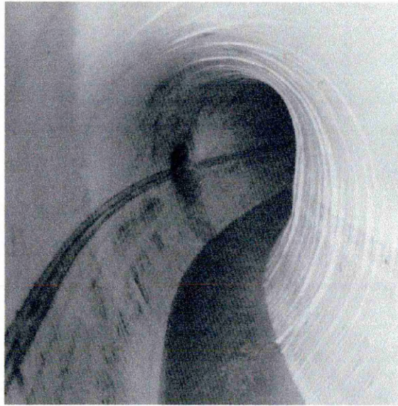
Figure 1.4: A CIP lined sewer.
