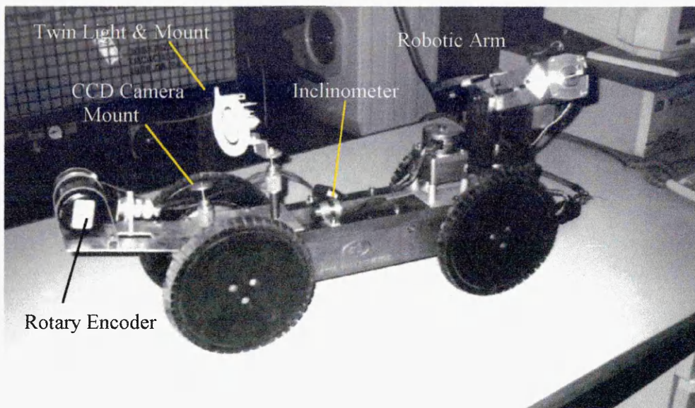
Figure 4.2: Tractor Unit & RetroFit Modules
