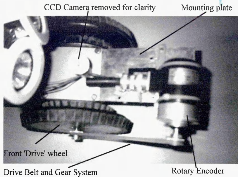
Figure 4.8: British Instruments Rotary Encoder – Plan View
