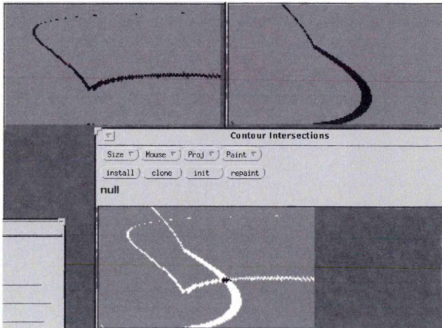
g. Isoluminance contours on the direct and reflected illumination reflectance maps and their intersection, \rho = 90 , d = 3.032
