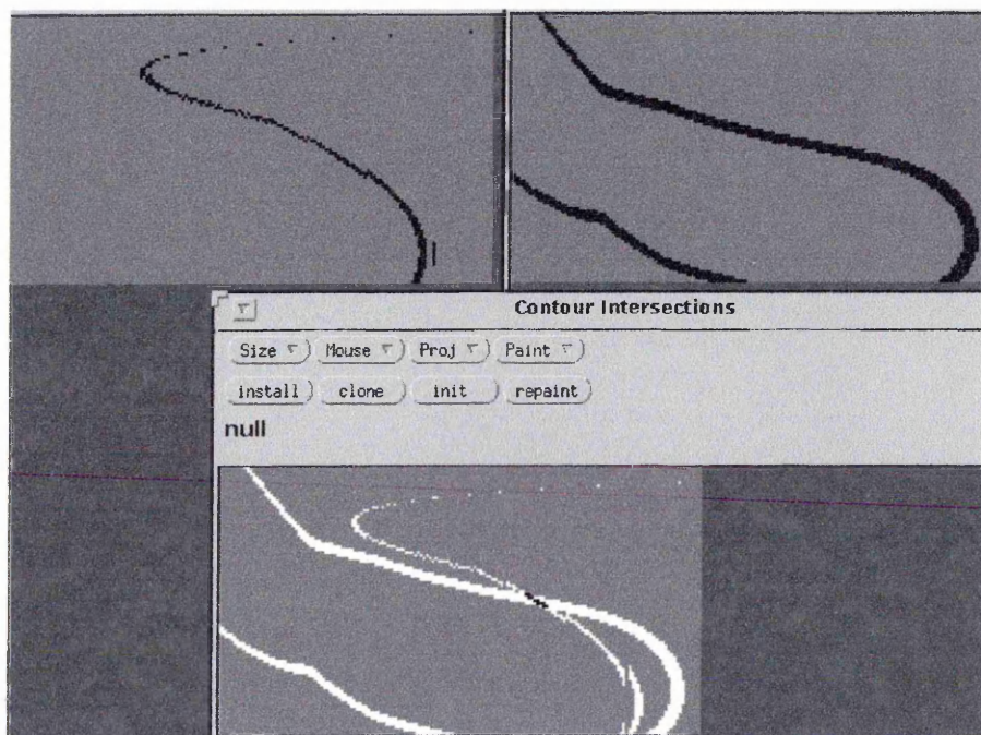
a. Isoluminance contours on the direct and reflected illumination reflectance maps and their intersection, \rho = 45 , d = 3.453
