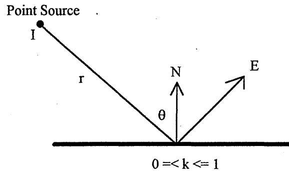
Figure C.1: Lambertian Reflectance
