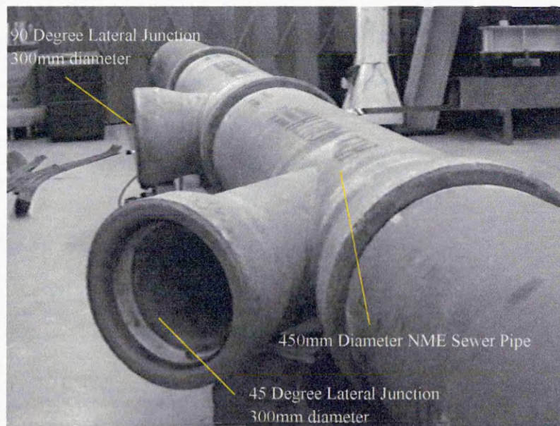
Figure 4.3: Laboratory Based Pipe Testing Rig
