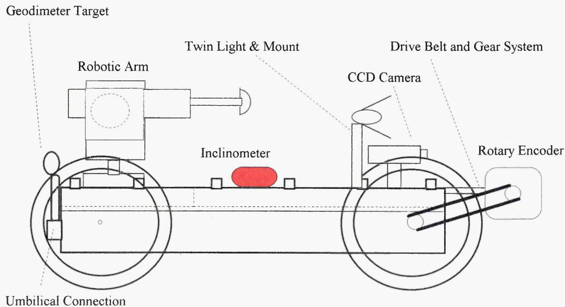
Figure 4.1: Retrofit Proposals for Cost Effective Sewer Robot
