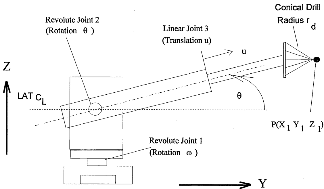
Figure 3.5c: Proposed Arm Configuration – On Target Elevation
