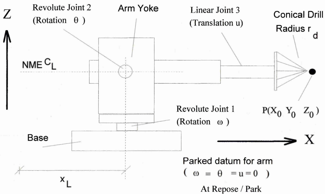
Figure 3.5b: Proposed Arm Configuration - Repose / Park Elevation
