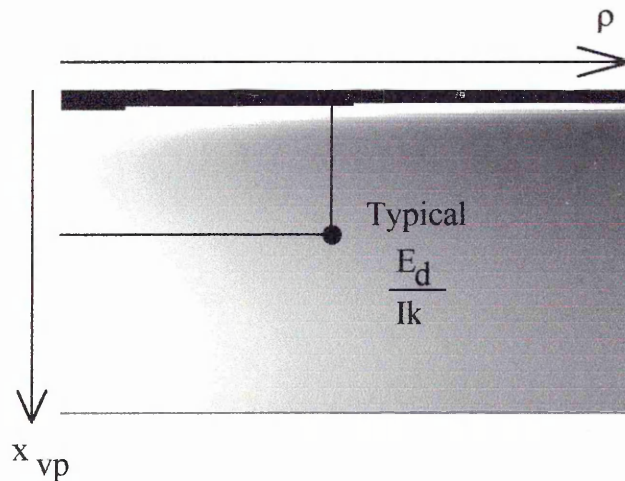
Figure 6.14. Surface Luminance Values Predicted by Direct Illumination Model
