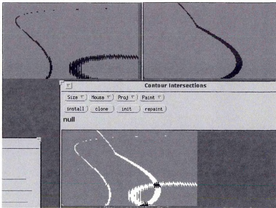
f. Isoluminance contours on the direct and reflected illumination reflectance maps and their intersection, \rho = 90 , d = 3.349
