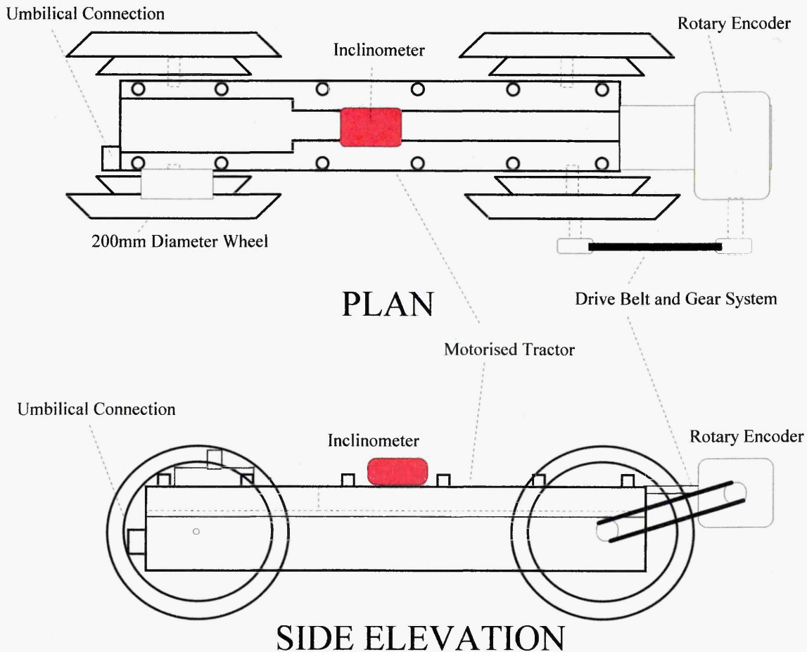
Figure 3.2: Rotary Encoder and Inclinometer System Components
