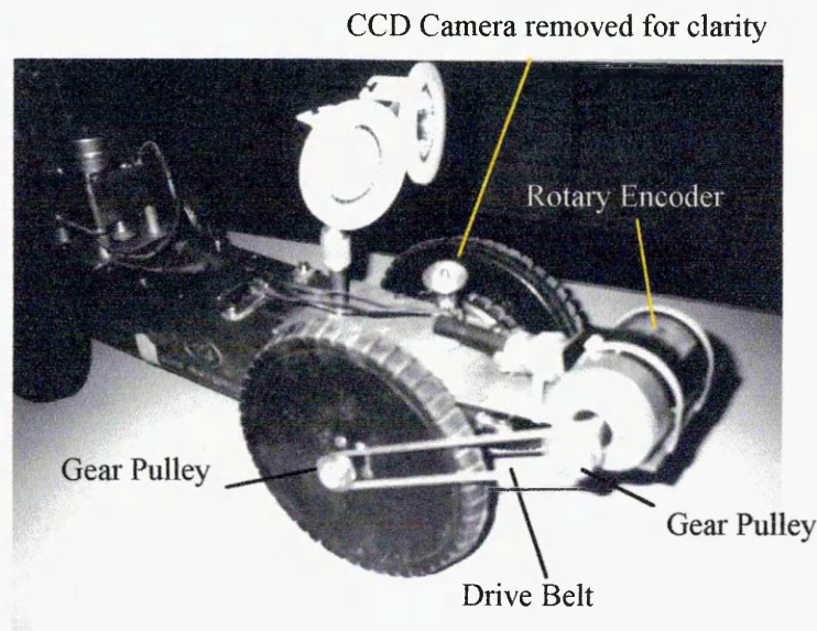
Figure 4.9: Rotary Encoder and Drive System - Elevation
