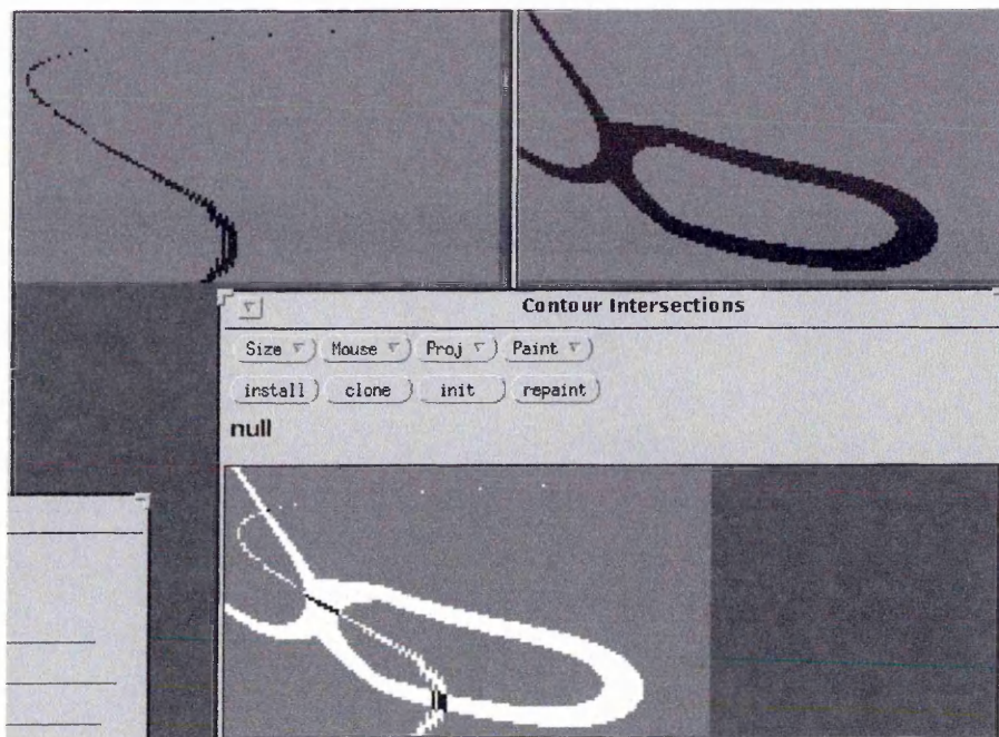
d. Isoluminance contours on the direct and reflected illumination reflectance maps and their intersection, \rho = 45 , d = 2.704
