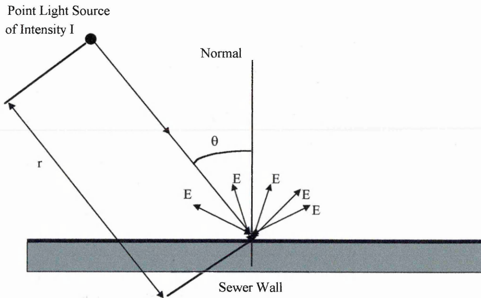
Figure 2.1: Lambertian Reflectance Characteristics
