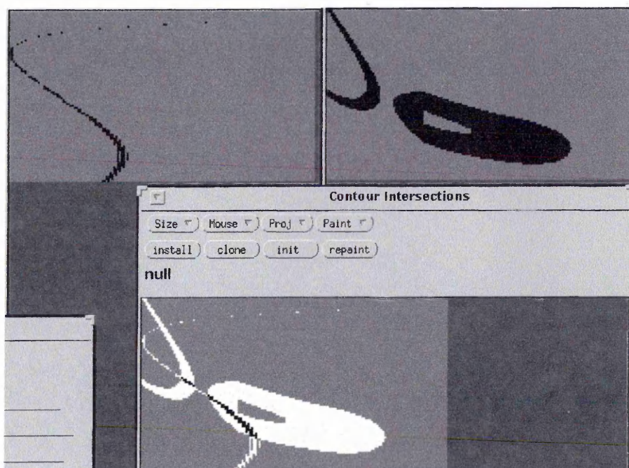
e. Isoluminance contours on the direct and reflected illumination reflectance maps and their intersection, \rho = 45 , d = 2.643
