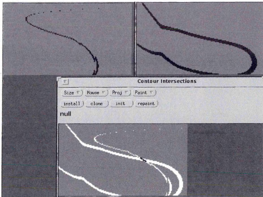
b. Isoluminance contours on the direct and reflected illumination reflectance maps and their intersection, \rho = 45 , d = 3.271
