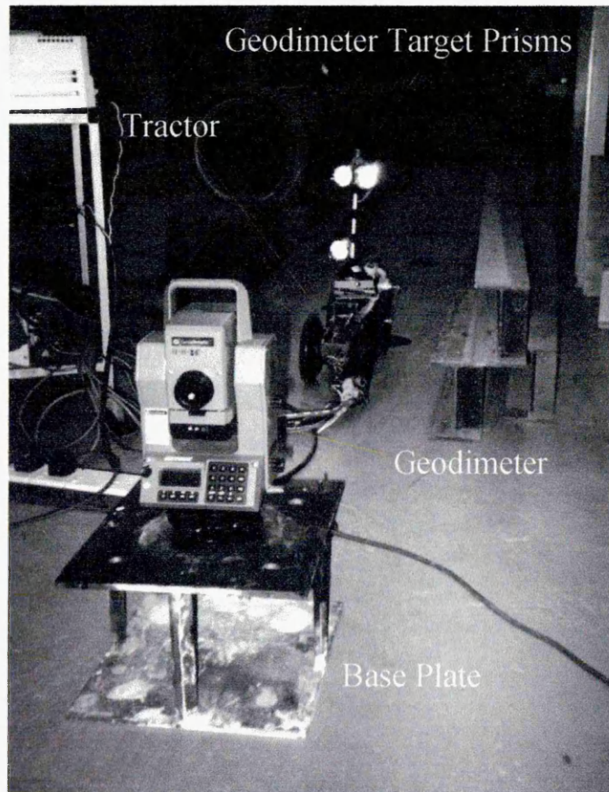
Figure 5.2: Geodimeter - Measuring Initial Datum Position
