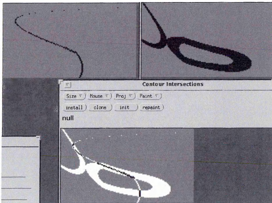
c. Isoluminance contours on the direct and reflected illumination reflectance maps and their intersection, \rho = 45 , d = 2.912
