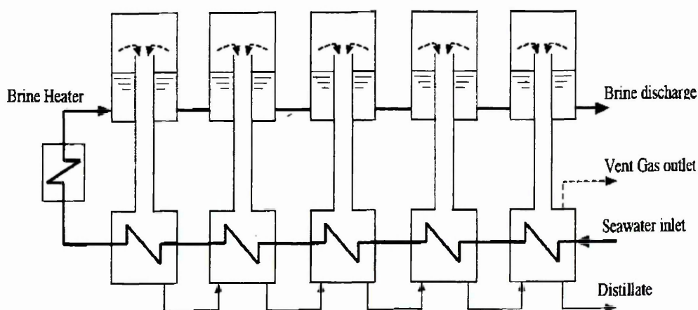
Figure 3.7: Schematic arrangement of the five-stage flash plant.
