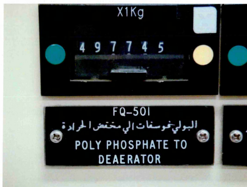
Figure F.14: Recorder of poly phosphate flow rate.
