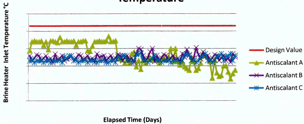
Figure 5.6: Measured Brine Heater Inlet Temperature
