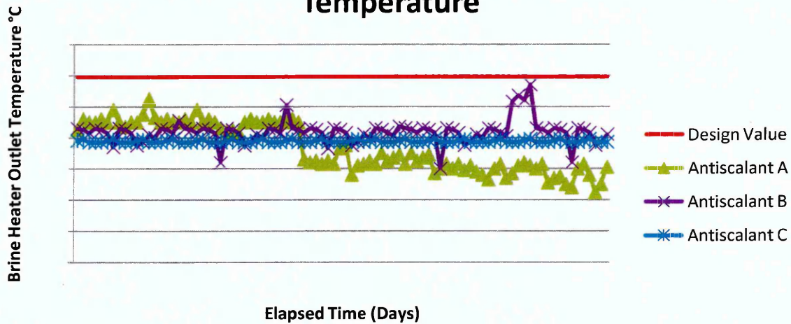
Figure 5.7: Measured Brine Heater Outlet Temperature
