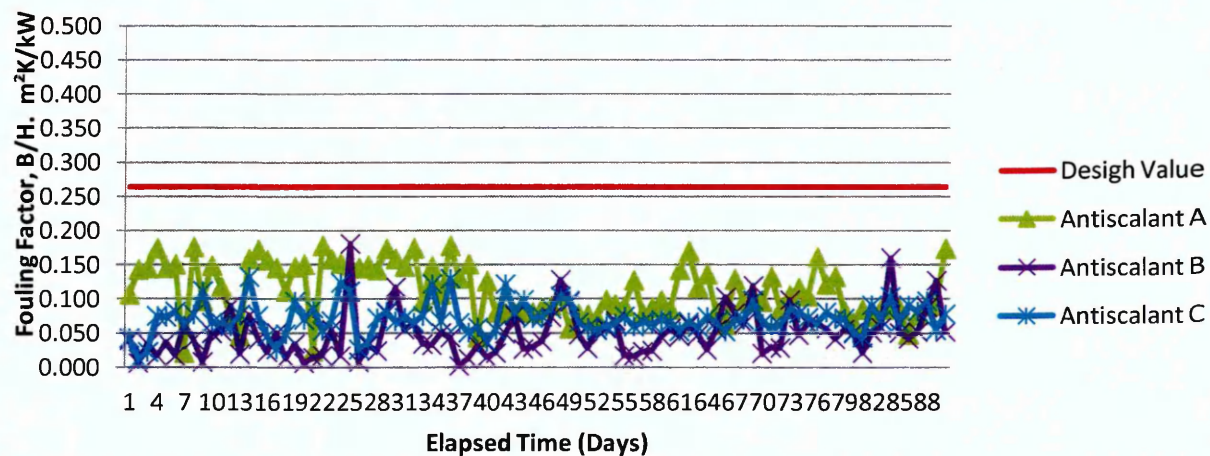
Figure 5.18: Calculated Fouling Factor, B/H.
