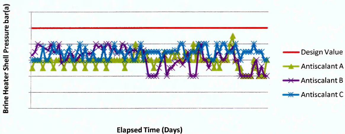
Figure 5.5: Measured Brine Heater Shell Pressure
