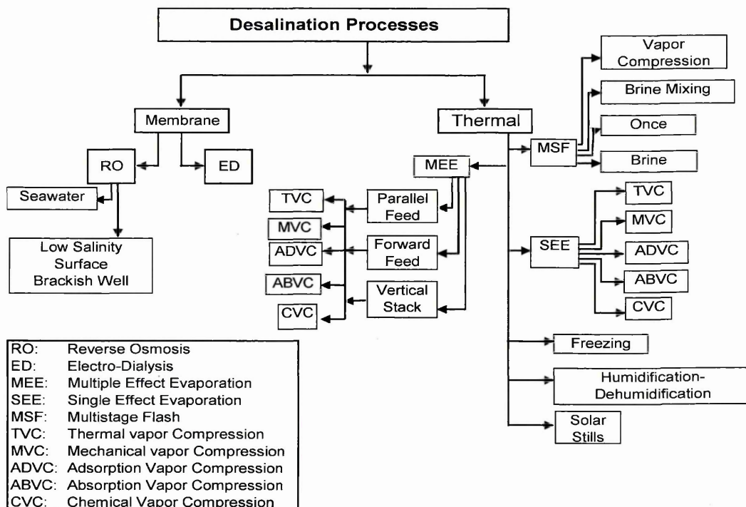
Figure 1.5: Classification of thermal and membrane desalination processes (11).
