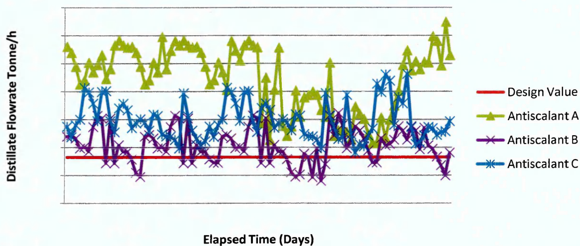
Figure 5.4: Measured Distillate Flowrate
