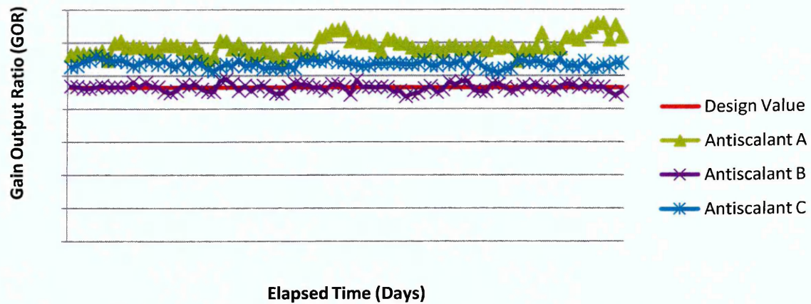
Figure 5.13: Calculated Gain Output Ratio (GOR)
