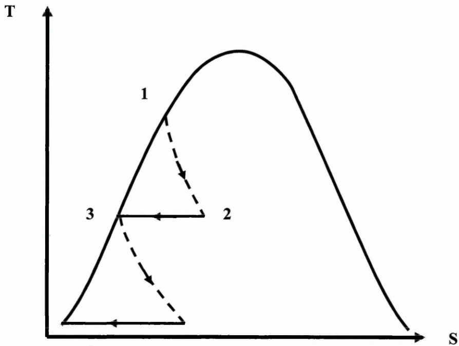
Figure 3.1: T-s diagram for the flashing process.
