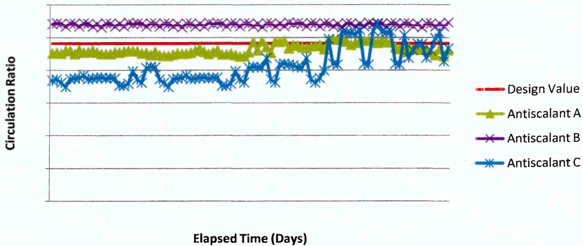
Figure 5.11: Calculated Circulation Ratio
