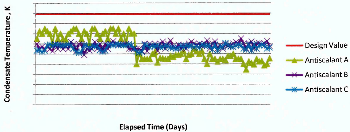
Figure 5.8: Measured Condensate Temperature
