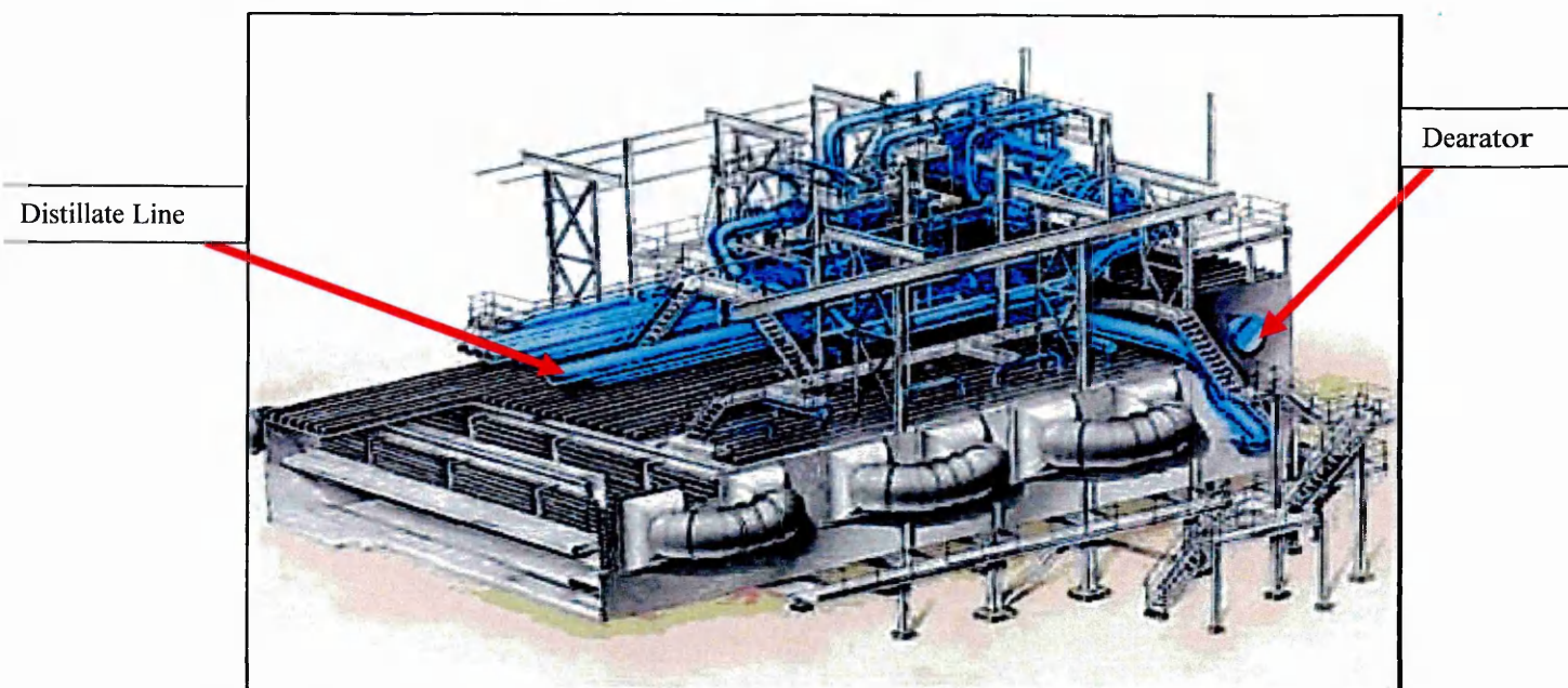
Figure 3.4: Schematic of a typical multistage flash desalination plant (11).
