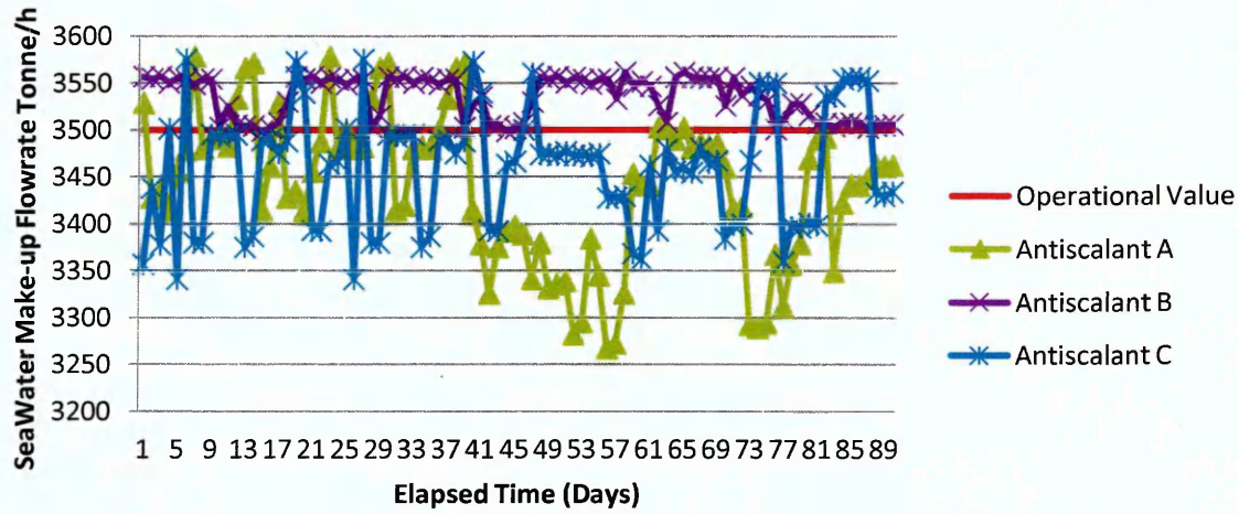
Figure 5.2: Measured Make-up Flowrate
