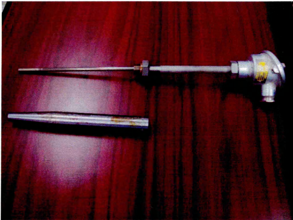
Figure 4.3: Photo of the thermo-couple and its thermo-well for measurement instrumentation (39).
