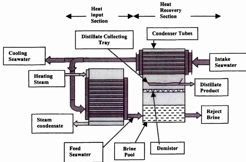
Figure 3.9: Once-through MSF desalination plant (28).
