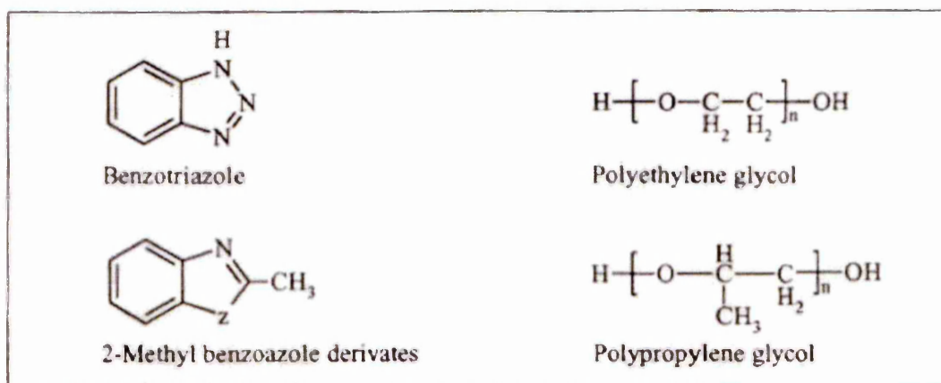
Figure C.2: Corrosion inhibitors (left, z=O: benzoxazole, z=N: benzoimidazole, z=S, Benzothiazole and z=Se: benzoselenazole) and antifoaming (right) (46).
