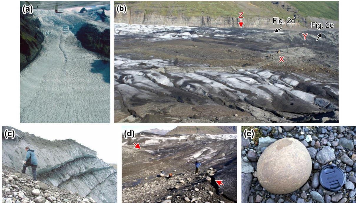
Figure 2: (a): View of the icefall and upper tongue. (b): View over the central area of the terminus (see Fig. 1(a)). Ice flow is towards lower right. Darker areas of ice have superficial cover from melt-out of dispersed englacial ash and tephra deposits. Medium-toned areas reflect thicker debris cover, comprising clasts of variable size and morphology, including material indicative of fluvial, subglacial and supraglacial transport. Light-toned debris regions include conspicuous transverse ridges or localised accumulations of thick debris (X, Y, Z) with a large proportion of large-calibre rounded and well-rounded (RWR) clasts that are commonly striated. (c) and (d): Debris bands emergent within and upglacier of debris accumulation Y (see (b)). Arrows in (d) indicate the debris band location. (e): A well-rounded clast, photographed in the proglacial area, exhibiting striae and a percussion fracture, and therefore definitive evidence of post-fluvial active glacial (i.e. subglacial) transport.
