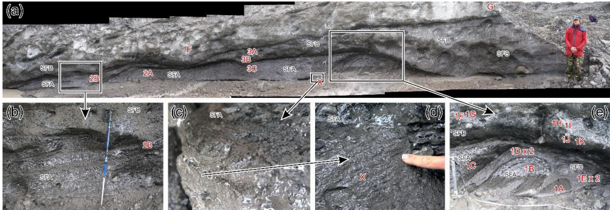
Figure 5. (a): Detail of basal ice section in Fig. 4(e) showing facies types (black text; see Table 1) and isotope sample locations (red text). (b): Stratified facies exhibiting folding (tectonic thickening). (c), (d): Stratified facies situated above frozen subglacial diamicton, showing uniform upglacier dip of clean ice and debris-rich laminae both above and below the ice-diamicton boundary; X indicates the diamicton isotope sample location. (e): Several tight folds in stratified solid facies (SFD) ice containing stratified facies (SFA) ice (isotope sample locations are again indicated).
