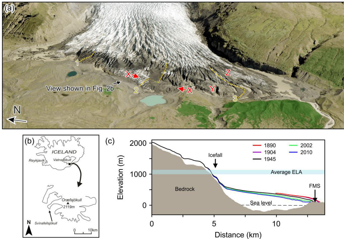
Figure 1: (a): Oblique view of the terminus from LiDAR and aerial photography obtained in 2009. X and X 1 indicate the location of a prominent transverse supraglacial moraine shown in Fig. 2b. Y and Z are other prominent spreads of large calibre supraglacial debris. 1 to 3 indicates the locations of three structural surveys (see section 4.2). (b): General location of Svínafellsjökull. (c): Longitudinal profiles of Svínafellsjökull between 1890 and 2010 and average ELA determined from snowline altitude in MODIS imagery (redrawn from Hannesdóttir et al., 2012). FMS = frontal moraine system.
