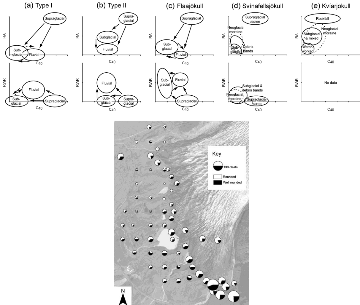
Figure 18. Above: Clast form co-variance summary plots. (a) and (b): Two main co-variance types identified by Lukas et al. (2013) from a large temperate glacier dataset (Type I: mountain glaciers; Type II: high-mountain glaciers). (c): Co-variance plots for Flaaajökull showing a higher proportion of RWR clasts in subglacial origin sediments than is typical arising from transfers of material between subglacial and fluvial transport paths (Lukas et al. 2013). (d): Co-variance plots for Svínafellsjökull showing a less substantial but still marked proportion of RWR clasts in subglacial origin material and frontal moraines. Frontal moraine characteristics overlap notably with debris band characteristics. (e): Co-variance plot for Kvíarjökull redrawn from Spedding and Evans (2002) showing similar overlap between frontal moraine and ‘water-worked’ supraglacial material derived from englacial channel fill and debris-band melt out (cf. Swift et al. 2006). Below: Abundance of RWR clasts in the frontal moraine system at Svínafellsjökull determined by sampling of all surface clasts in a 25 m 2 grid. Symbol size is proportional to clast count and shows relative proportion of rounded and well-rounded clasts.
