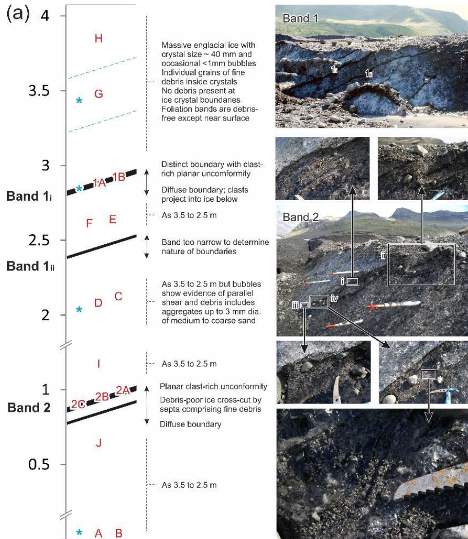
Figure 10. Vertical log through debris bands and adjacent ice at exposures 4 and 5 on survey 2. (a) Log through bands 1 to 3 at exposure 4 (see Fig. 6d). Left: Sedimentary log, showing location of isotope (letters) and ice crystal samples (* symbols), and major ice facies and band characteristics. Note the breaks in y-axis values. Right: Photos include close-views of several band characteristics (ice axe for scale). i: Sharp upper boundary between band ice below and firnified glacier ice above; ii: Fold in band ice beneath the main ‘active’ band; iii: Larger clasts at upper band surface, demonstrating strong fabric in ice flow direction; iv: Close view of stratified ice layering crossing clean ice sandwiched between upper and lower band surfaces. Stakes shown in the central photo of Band 3 were monitored for c. 10 days during summer 2007, but no displacement was observed.
