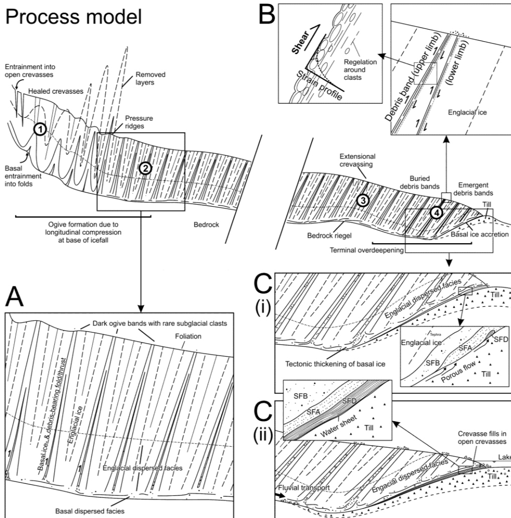
Figure 17: Process model illustrating the key proposed debris-rich glacial ice formation processes, debris transport pathways, and glaciological controls. 1. Entrainment into basal folds and surface crevasses at the ice fall. 2. Deformation below the ice fall further elevates basal material into dark-ogive bands (see detail in panel A). 3. Ice and subglacial water flow enters the terminal overdeepening. 4. Longitudinal flow compression produces thrusting along ogive-band foliation,
