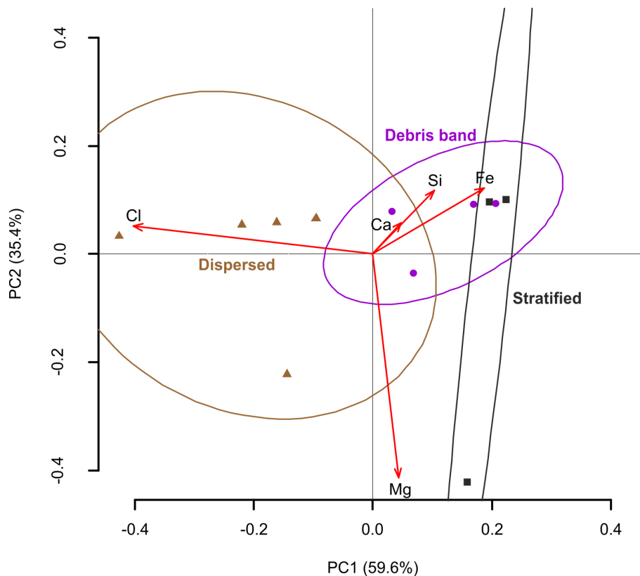
Figure 12. Biplot showing results of Principal Component Analysis of XRF element data from 2015 basal ice and debris band samples. Envelopes are drawn for a confidence interval of 95%. Leading elements for the differences were chlorine (Cl), which was more abundant in dispersed facies ice, and iron (Fe) and silica (Si), which were more abundant in stratified ice.
