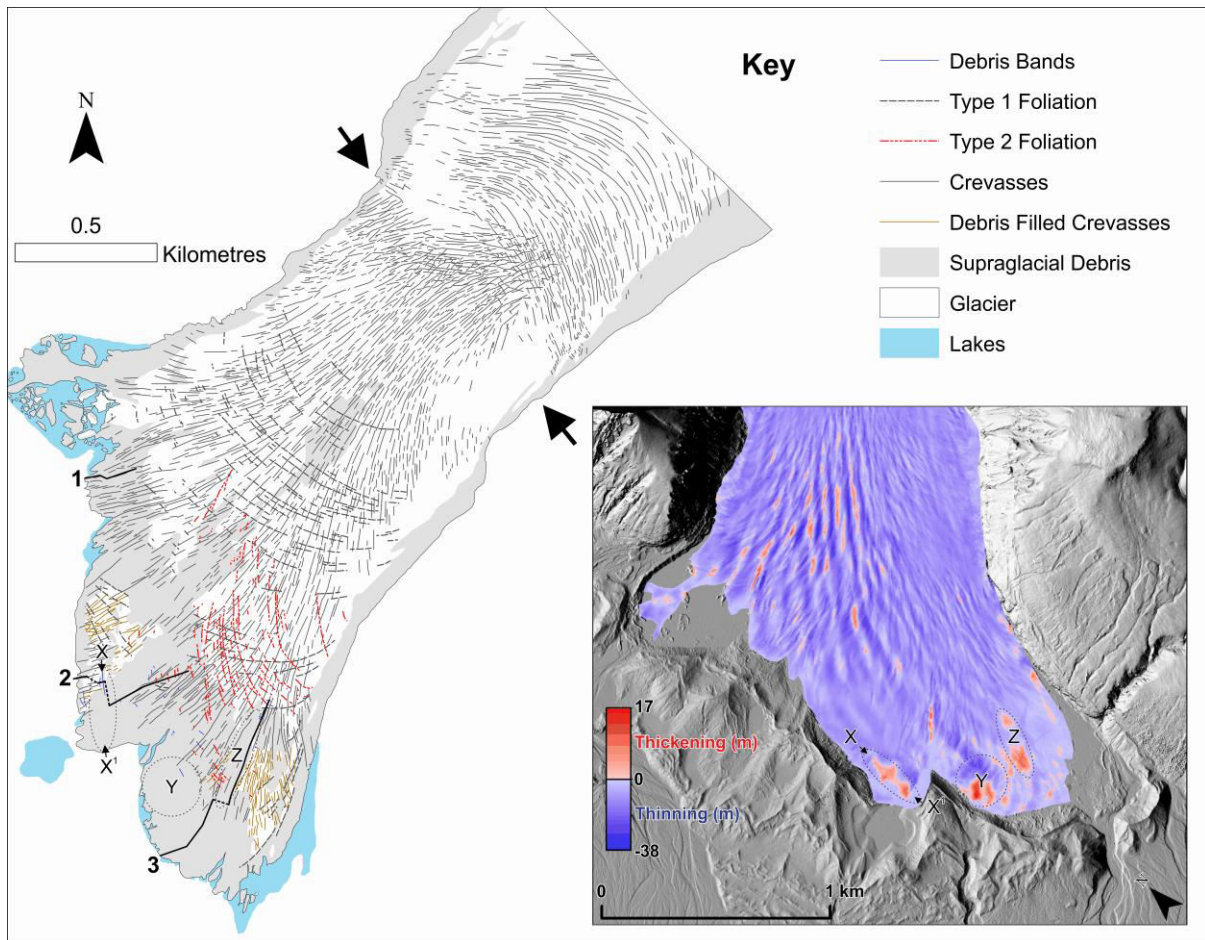
Figure 3: Structural map of the lower tongue of Svínafellsjökull. 1 to 3 mark the positions of the flow-parallel surveys shown in Fig. 1a. X–X 1 , Y and Z denote major surface debris spreads shown in Figs. 1a, 2a. Inset: Surface elevation change between 2007 and 2009 overlain on the 2009 LiDAR DEM hillshade. Areas of pronounced thickening (shown by red colouring) occur in the region of debris spreads X–X 1 , Y and Z. Other areas of thickening relate to antiphase crevasse and serac migration between the datasets, rather than in situ surface changes.
