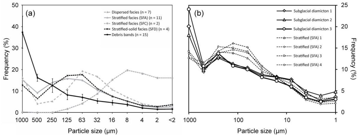
Figure 13: Sediment particle size distributions for debris band, basal ice, and subglacial diamicton samples. (a) Distributions for basal ice (Cook, 2006; Cook et al. 2010) and debris band samples (this study). Dispersed facies and stratified facies A and D are described in Table 1. Stratified facies C (cf. Cook et al. 2010) were observed to connect with ‘crevasse fill’ features (cf. Fig. 7). (b) Distributions of stratified facies ice A and subglacial diamicton samples (this study).
