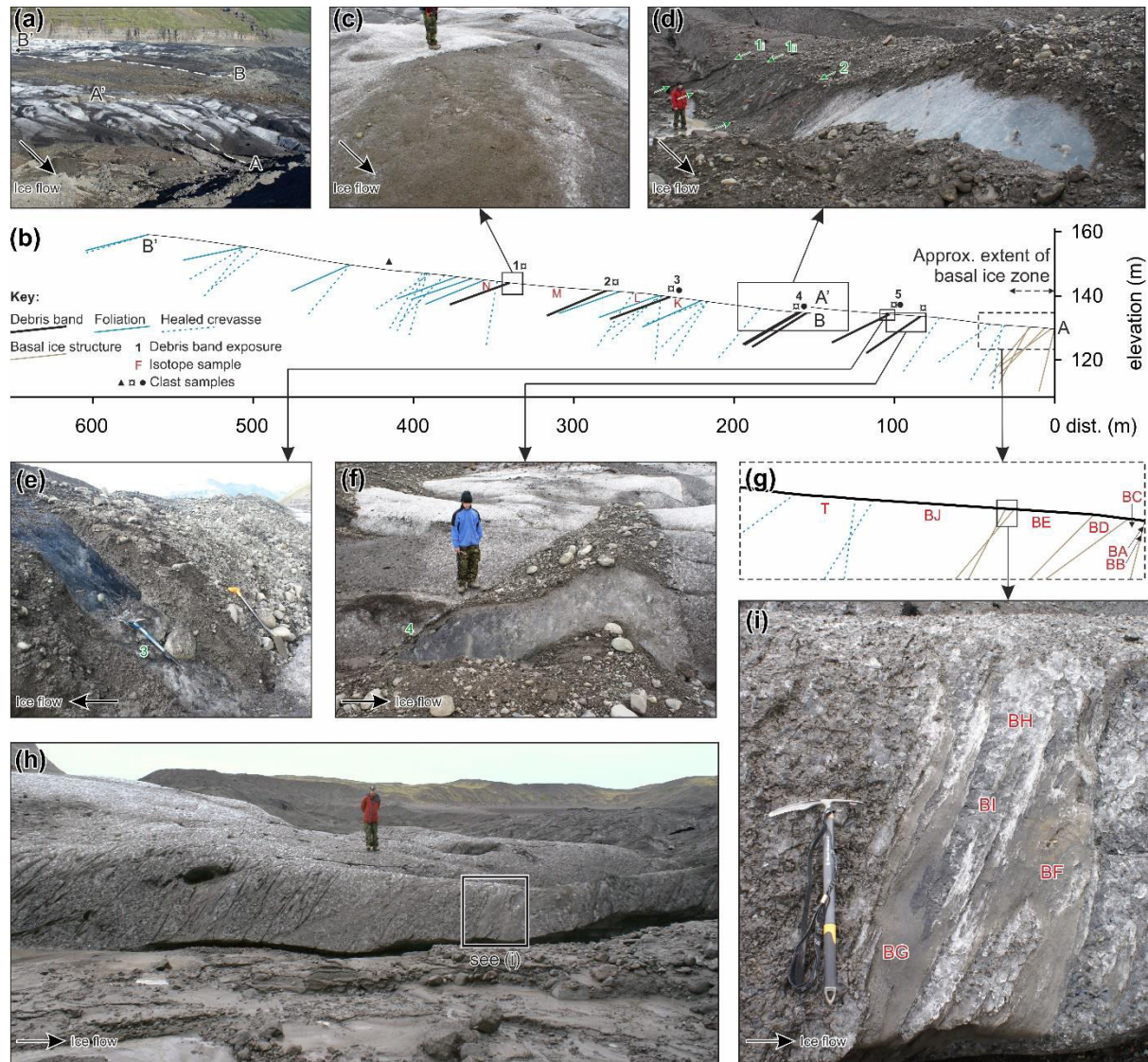
Figure 6. (a): View of central area of terminus showing survey 2. (b): Survey line elevation and key structures (see key). Isotope sampling locations indicated by coloured lettering. Clast sample symbols indicate supraglacial ( \blacktriangle ), debris band ( \boxtimes ), and band-origin supraglacial debris ( \bullet ) (see Fig. 15). (c) to (f): Examples of debris bands observed along the survey. A structural log (Fig. 10) encompassing bands 1 and 2 (see d) at exposure 4 and 3 and 4 (see e and f) at exposure 5 is described in the text. (g, h, i): Detail of basal ice section, also showing further isotope sampling locations.
