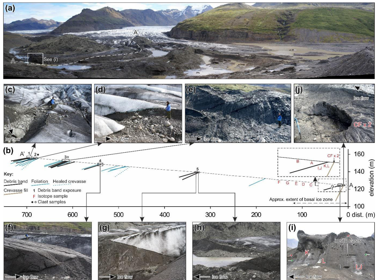
Figure 8. (a): View of southern area of terminus showing survey 3. (b): Survey line elevation showing foliation (blue), healed crevasse (blue dashed) and debris band (black) exposures (numbered). Isotope sampling locations of firnified glacier ice and basal ice are labelled A to L. Clast sample symbols indicate band-origin supraglacial debris clast form sample (●) (see Fig. 15) and rounded clast count (○) (Fig. 18b) locations. (c) to (h): Debris band exposures. (i): Basal ice section near terminus, also showing isotope sampling locations I to L. Red arrows indicate possible thrust of
