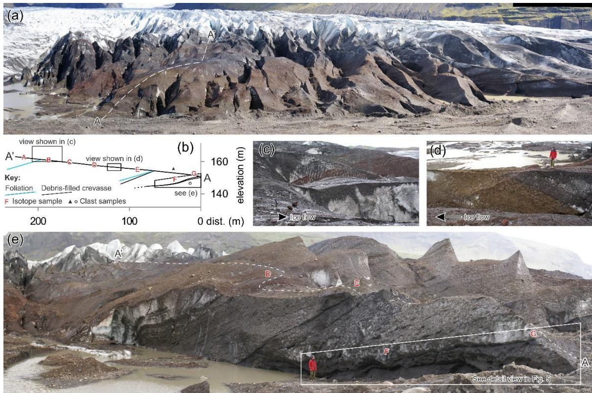
Figure 4. (a): View of the northern area of the glacier terminus (ice flow is towards the viewer). Line of survey is indicated A–A'. (b): Survey line elevation and isotope sampling locations (letters); the location and dip of prominent foliation (blue) and debris-containing features (black) is also shown. Clast sample symbols indicate supraglacial ( \blacktriangle ) and diamicton (pentagon) samples (Fig. 15). (c), (d): Views from the survey line showing foliation-parallel bands of ice defined by the colour of englacial debris (mainly tephra). (e): Context of the basal ice section shown in Fig. 4.
