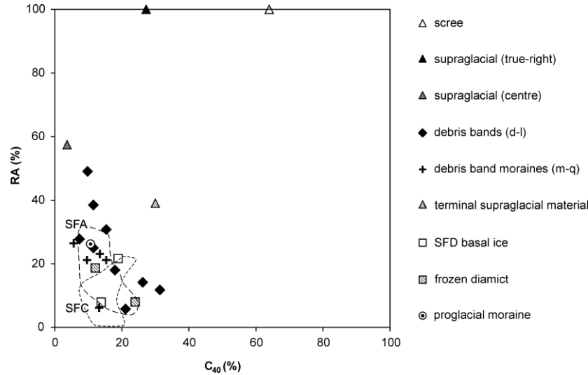
Figure 16: Bivariate plot of C_{40} against Relative Angularity (RA) for clast samples shown in Fig. 15. SFD indicates the stratified solid facies basal ice clast sample obtained in 2005 (Fig. 9). Envelopes of stratified basal ice clast samples from Cook et al. 2011b are shown (dashed lines) for comparison (stratified basal ice subfacies A is formed by regelation; subfacies C is formed by freeze-on of supercooled water as a consequence of glaciohydraulic supercooling).
