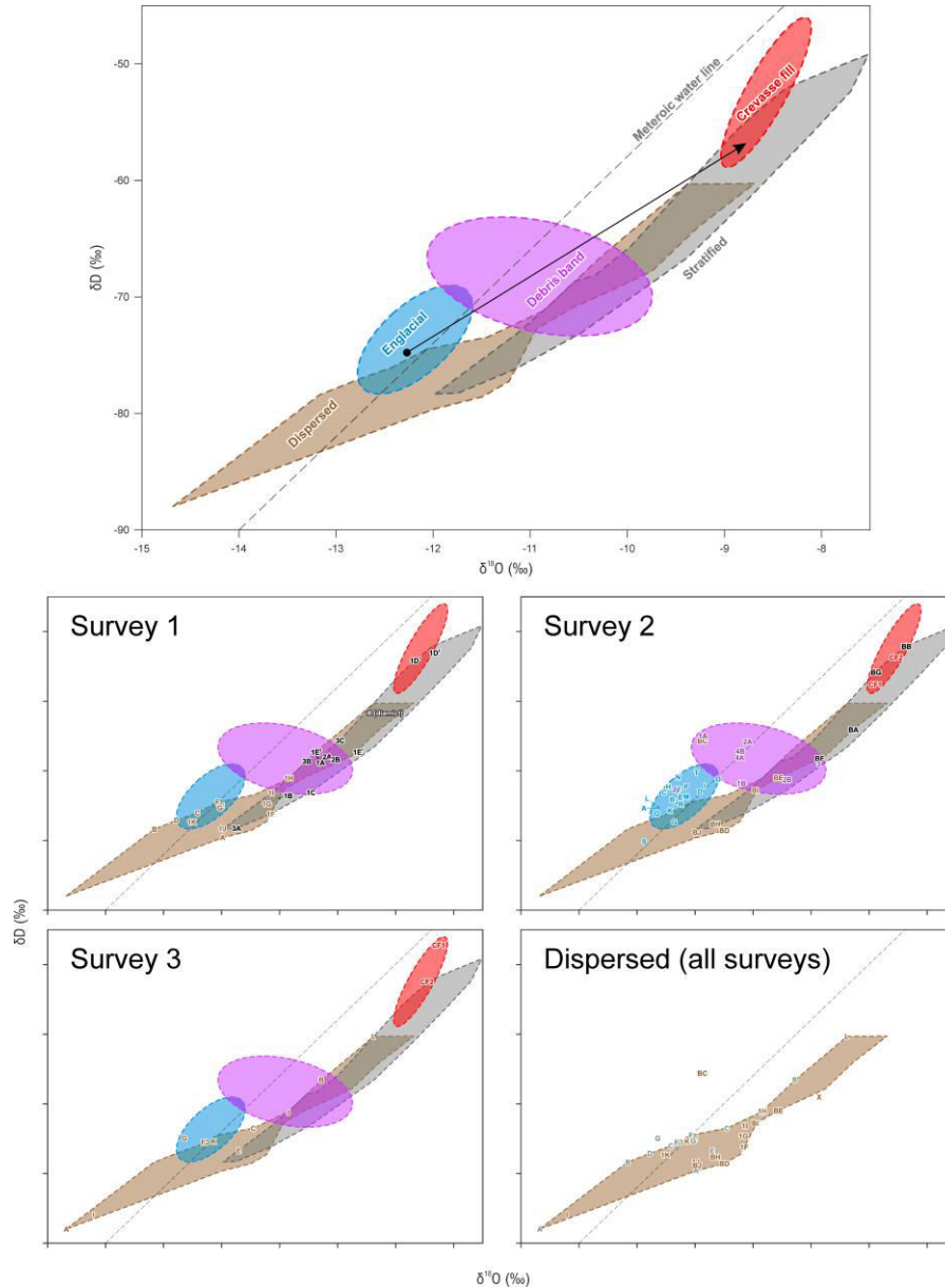
Figure 11: Isotopic composition ( \delta^{18}\text{O} against \delta\text{D} ) of debris band ice, firnified glacier ice and basal ice facies sampled in 2005 and 2007. Upper diagram summarises sample envelopes. The black arrow shows predicted offset in composition after open system refreezing of ice with an average firnified glacier ice composition (cf. Cook et al. 2010). Lower diagrams show compositions of samples on individual surveys. The meteoric water line has been adjusted to plot through the samples from Svínafellsjökull. Englacial samples containing dispersed tephra (see text) are included in the dispersed envelope in all diagrams and are shown plotted separately in green in the final panel.
