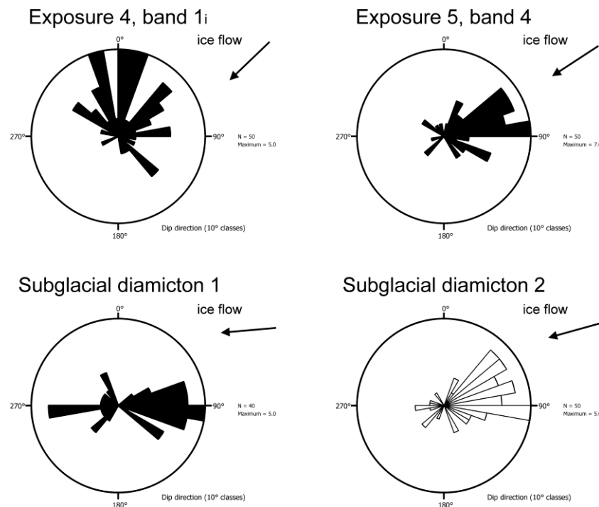
Figure 14: Uni-directional rose diagrams showing clast orientation and dip for samples of clasts from two debris bands and two frozen subglacial diamicton units. The approximate direction of ice flow, determined by analysis of aerial photography, is shown for reference.
