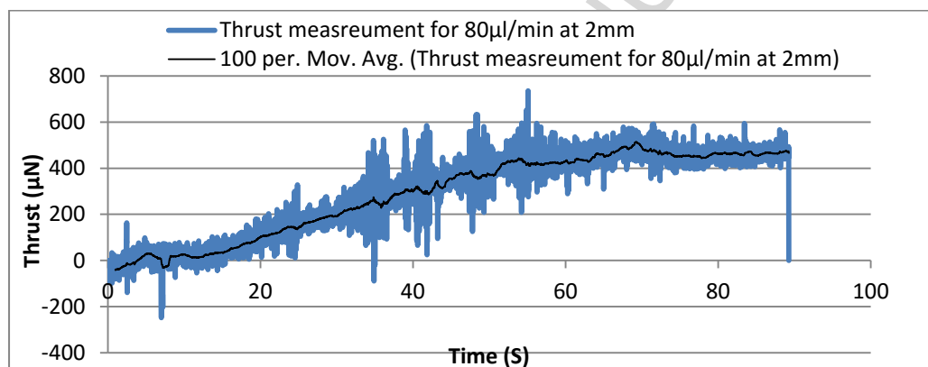
Figure 15 Thrust measurement for 80 \mu\text{l}/\text{min} propellant flowrate measured at 2mm distance.
