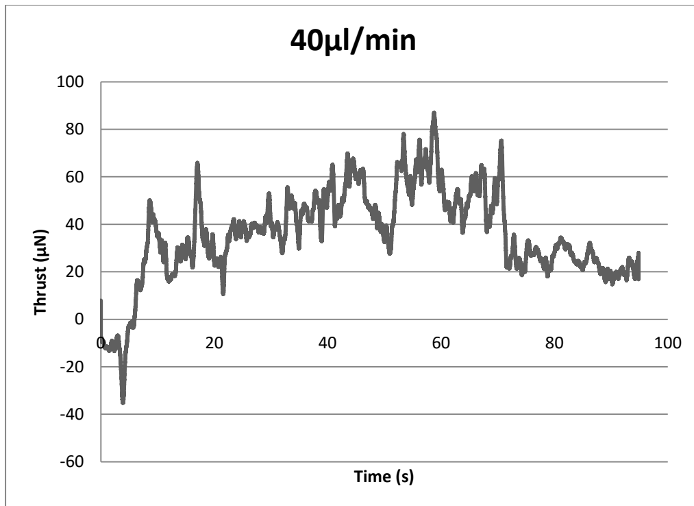
Figure 17 Thrust measurement results for 40 \mu l/min flowrate
