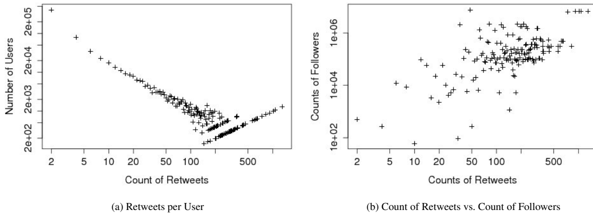
Fig. 5. Distribution of Retweets per User and Retweets vs. Followers.
