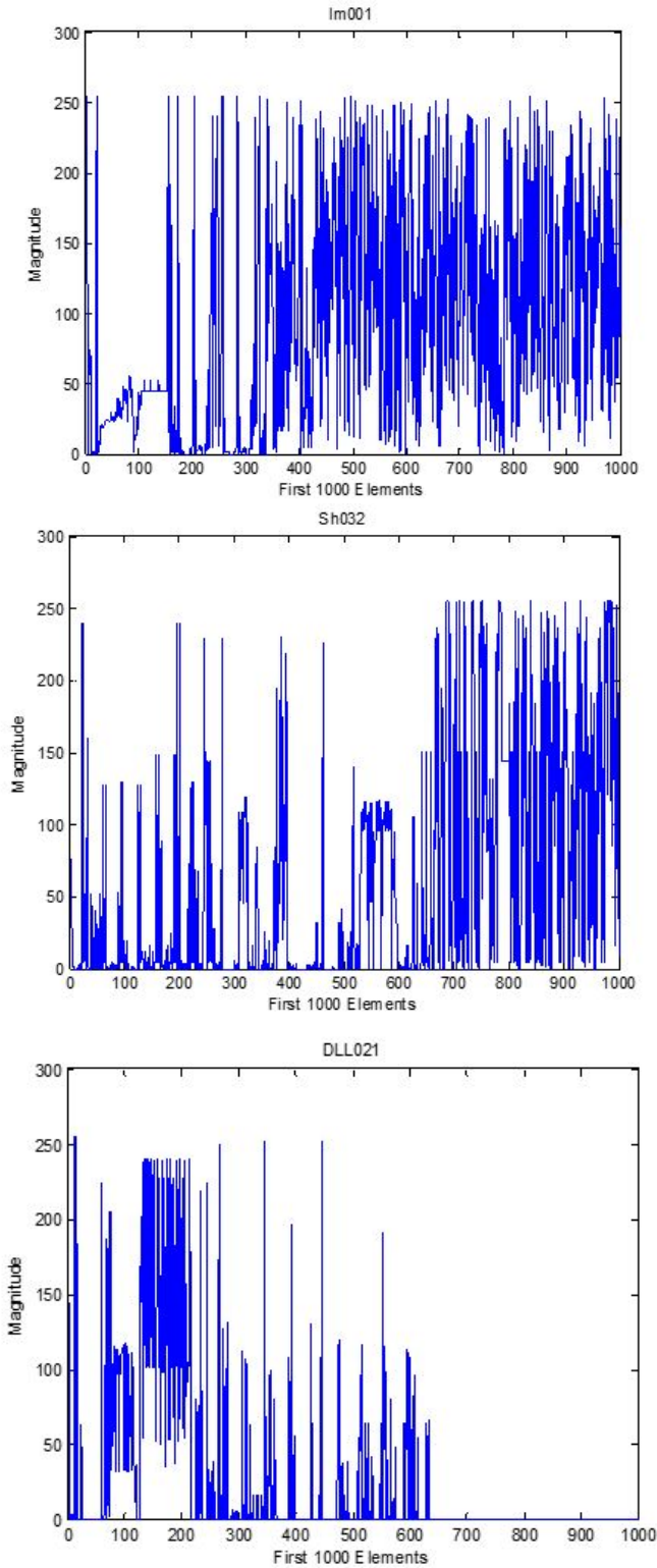
Fig. 1. Example plot of 1,000 data points of collected data (padded with zeros where required). Top: a jpeg image, middle: a shellcode, bottom: a DLL.
