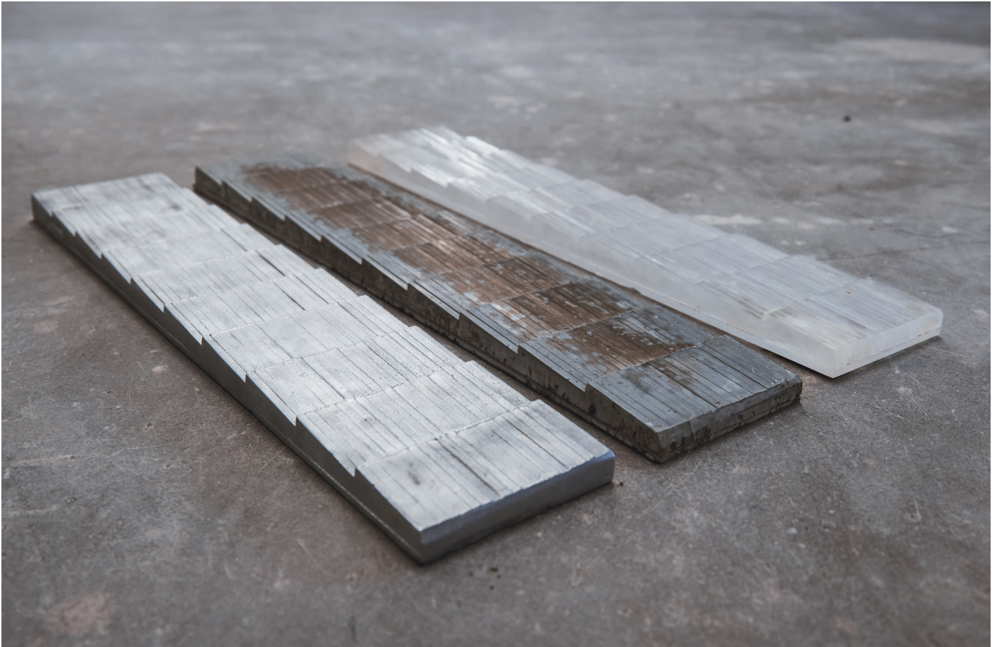
Material exploration into cast aluminium, cast concrete and acrylic (Bell, 2016)
