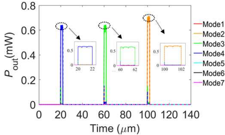
Figure 3. Self-mixing response at three different frequency bands generated by LFI with thermal modulation in a coupled-cavity THz QCL: (a) the passive cavity driving pulses (b) the active cavity driving pulses (c) the time varying emission frequency (d) the output power of the coupled-cavity THz QCL with optical feedback when target reflectivity R = 0.7 (solid lines) and no optical feedback (dashed lines).
