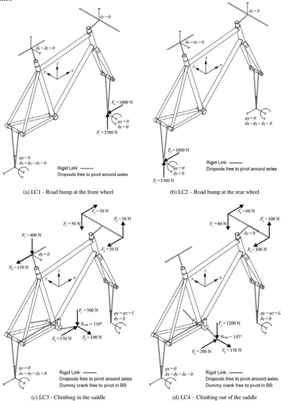
Fig. 2. Free body diagrams for the four load cases simulated in this study, based on measurements presented in the literature. Note \theta_{crank} is measured anti-clockwise from the vertical z-axis.
