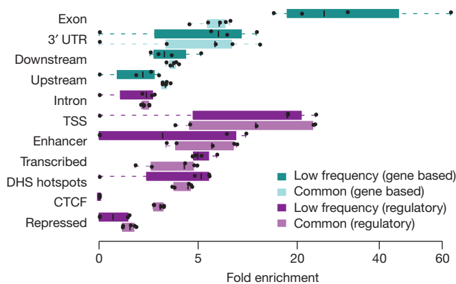
Figure 5 | Enrichment of single-marker associations by functional annotation in the UK10K-cohorts study. Distribution of fold enrichment statistics for single-variant associations of low-frequency (MAF 1–5%) and common (MAF \geq 5%) SNVs in near-genic elements or selected chromatin states and DNase I hotspots (DHS). Boxplots represent distributions of fold enrichment statistics estimated across the five (out of 31 core) traits where at least 10 independent SNVs were associated with the trait at 10^{-7} P value (permutation test) threshold (HDL, LDL, TC, APOA1 and APOB). Chromatin state and DHS regions were inferred from ENCODE data in a liver cell line, HepG2, which is informative for lipids. Promoter and 5' UTR are not shown, but corresponding statistics are given in Supplementary Table 12.
