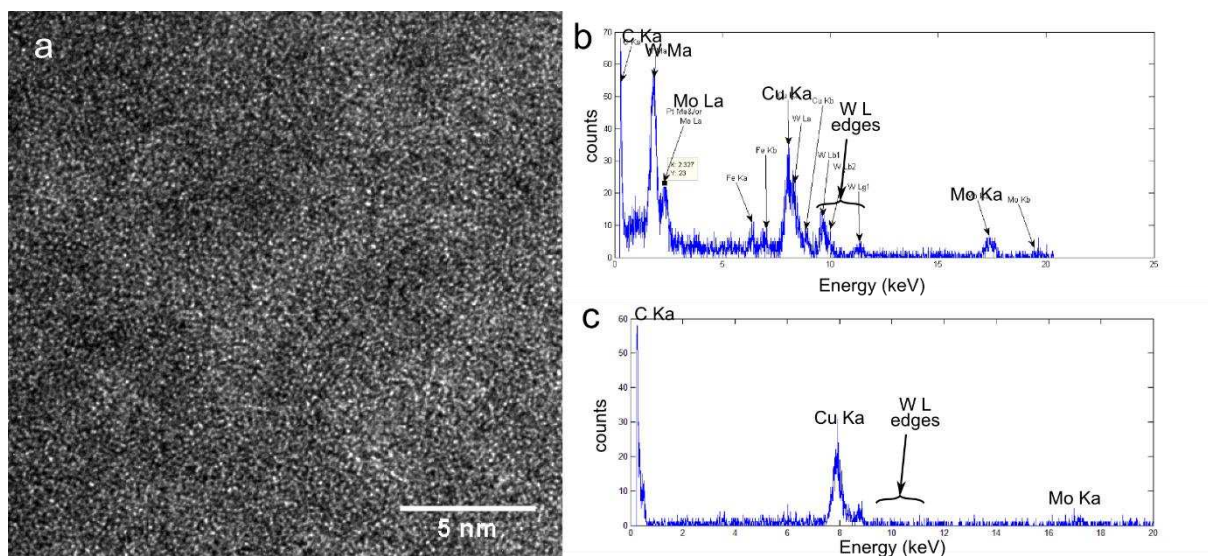
Figure 2 (a) HRTEM image showing onion-like parts in clusters. (b) EDS spectrum from cluster in thinner sample made later (not this sample, but deposited by the same procedure). (c) EDS from the matrix in this sample.
